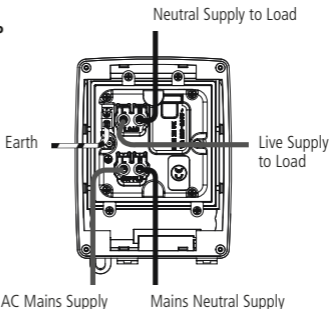
Figure 12 TGV104NP
