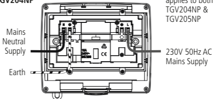
Figure 13 TGV204NP
