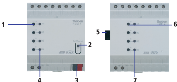
HMG 4 Basic device
