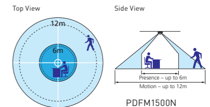
PDFM1500N detection range and coverage.
