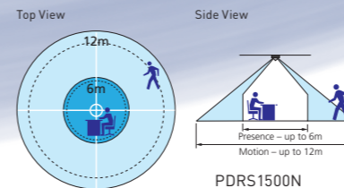
PDRS1500N detection range and coverage.
